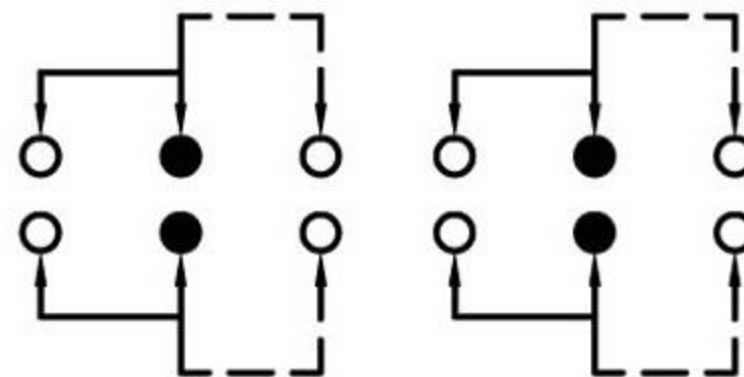
SCHEMATIC (NON-SHORTING)
